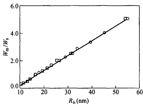
Fig. 2 Polymer/stabilizer weight ratio ( W_m/W_s ) dependence of hydrodynamic radius R_h of polystyren nanoparticles
